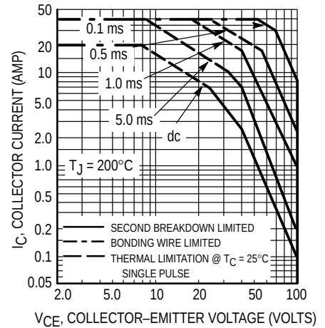
Figure 7. 2N6284, 2N6287
