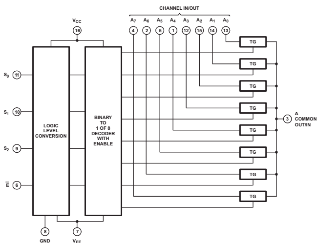
Functional Diagram of HC4051 and HCT4051
