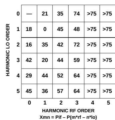
Figure 8. Harmonic Intermodulation Suppression (dB Below Desired Output) RF at 1\text{ GHz} , LO at 0.752\text{ GHz} , IF at 0.248\text{ GHz} .
