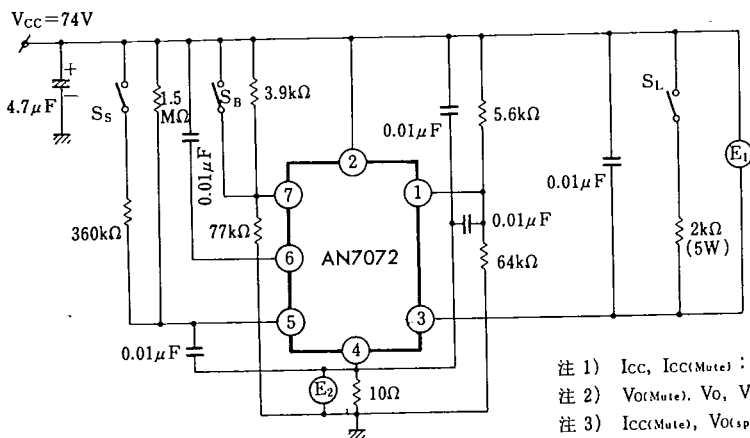
Test Circuit 1
