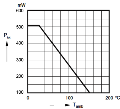
Admissible Power Dissipation Vs. Ambient Temperature
