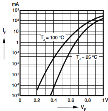
Forward Characteristics
