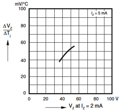
Temperature Dependence of Zener Voltage Vs. Zener Voltage
