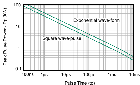
Figure 2. Non-repetitive peak pulse power rating curve
