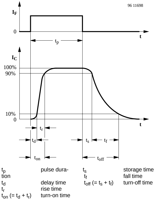
Figure 5. Switching times
