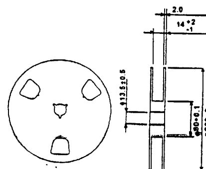
330 mm/13" Reel
