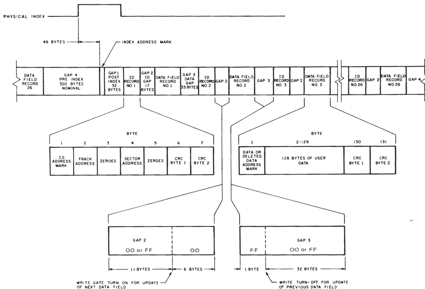
FIG.13 TRACK FORMAT
