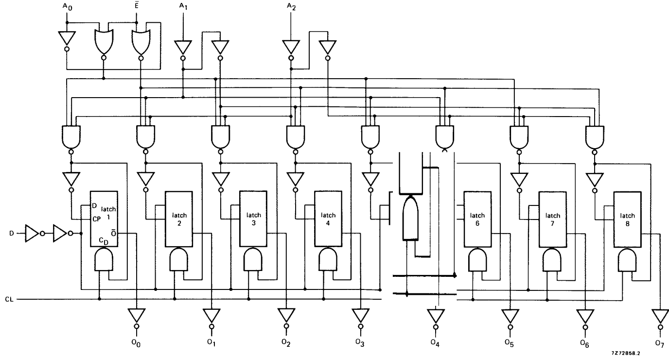
Fig.3 Logic diagram.
