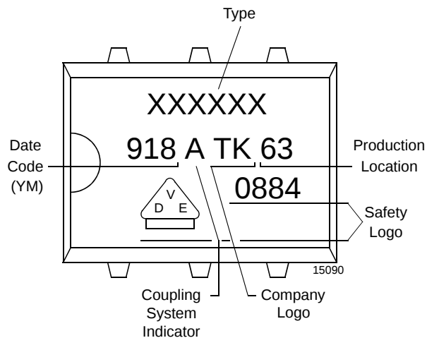
Figure 13. Marking example
