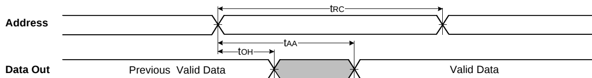
TIMING WAVEFORM OF READ CYCLE(1) (Address Controlled, \overline{\text{CS}}_1=\overline{\text{OE}}=V_{\text{IL}} , \text{CS}_2=\overline{\text{WE}}=V_{\text{IH}} )
