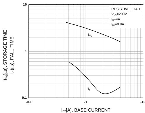
Figure 5. Switching Time
