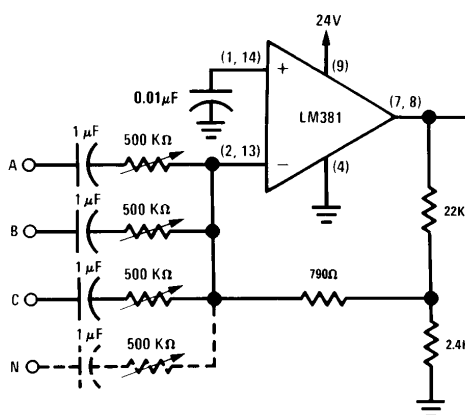
Audio Mixer
