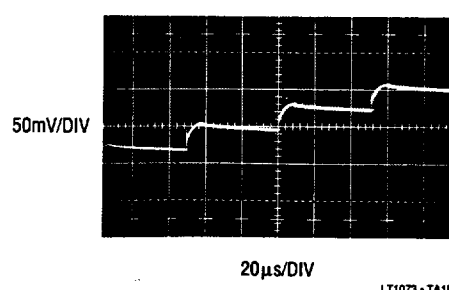
Figure 5. OS-CON
