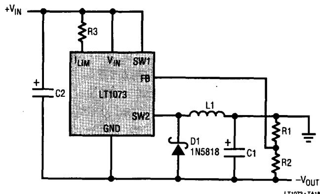
Figure 8. Positive-to-Negative Converter
