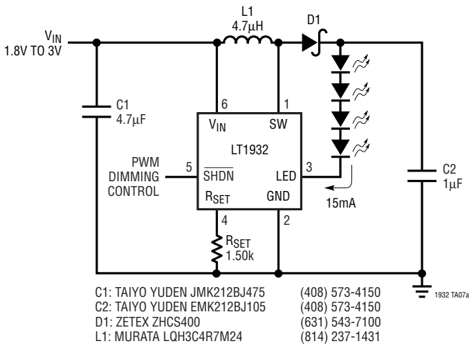
2-Cell Driver for Four White LEDs
