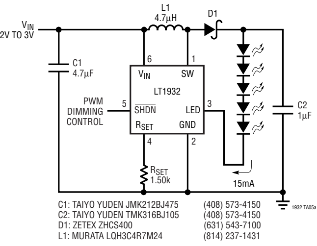
2-Cell Driver for Five White LEDs
