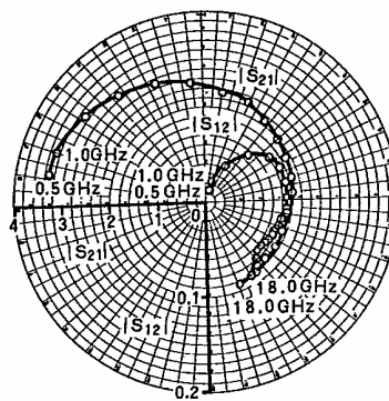
S_{12}, S_{21} vs. f
