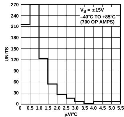
Figure 30. TCV_{OS} Distribution (J Package)
