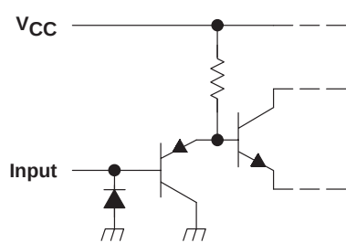
equivalent schematic of each input
