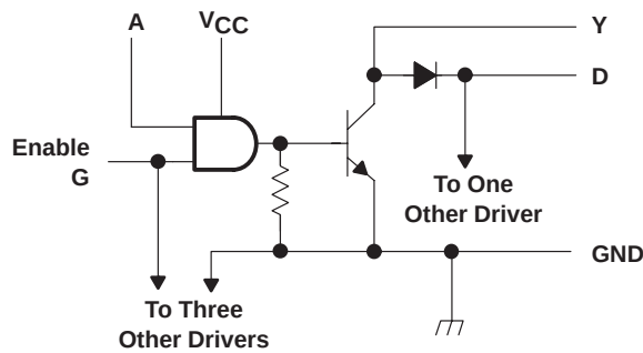
logic diagram (positive logic, each driver)
