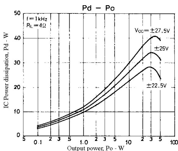
Figure 2. STK4028V Pd – Po ( R_L = 4\Omega )
