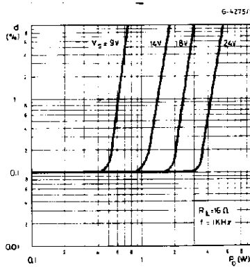
Figure 4. Distortion vs. output power ( R_L = 16Ω )
