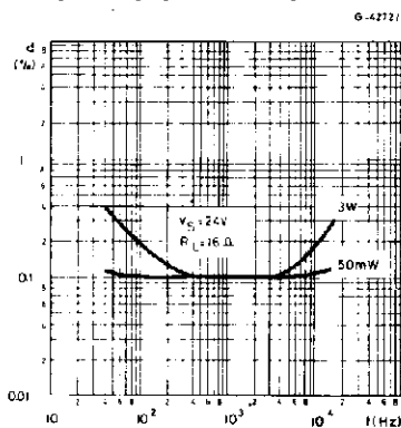
Figure 7. Distortion vs. frequency ( R_L = 16Ω )
