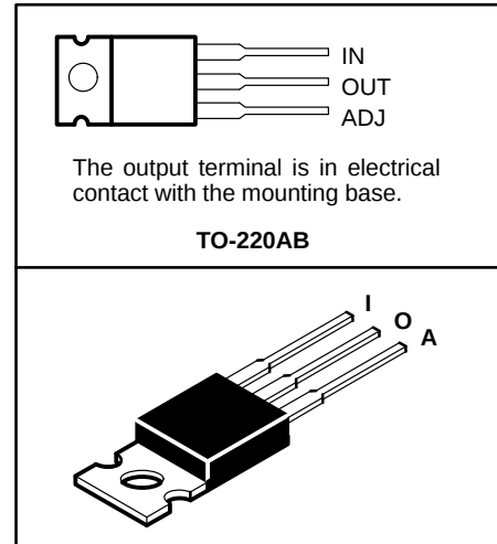
KC PACKAGE (TOP VIEW)
