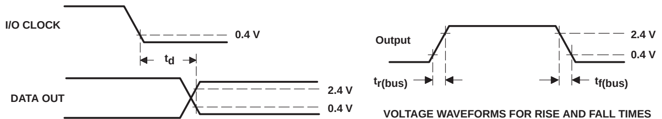
VOLTAGE WAVEFORMS FOR DELAY TIME
