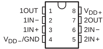
TLC2272 D, JG, P, OR PW PACKAGE (TOP VIEW)
