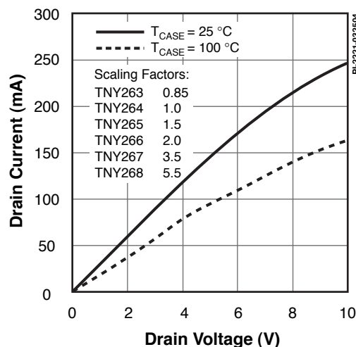
Figure 27. Output Characteristic.
