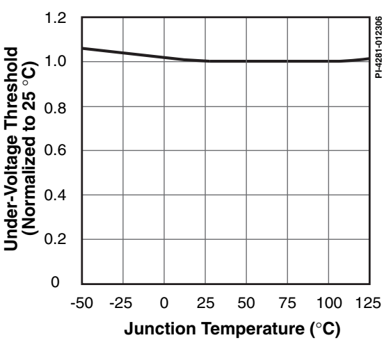
Figure 27. Undervoltage Threshold vs. Temperature.
