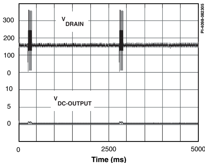
Figure 6. Auto-Restart Operation.
